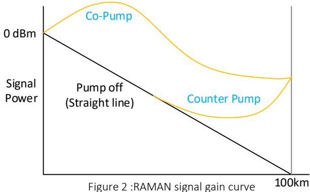
Figure 2 :RAMAN signal gain curve
